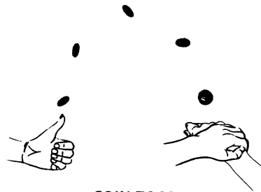
COIN TOSS
