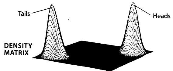
COIN TOSS
