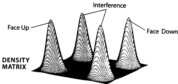
COHERENT SUPERPOSITION
