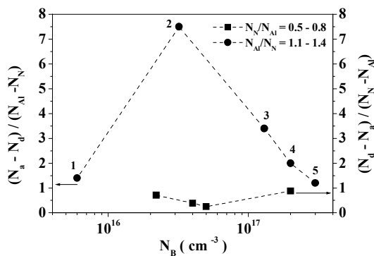
Fig. 1. The ratio of net acceptor concentration ( N_a - N_d ) to concentration difference ( N_{AI} - N_N ) vs. boron concentration ( N_B ) for the samples with N_{AI}/N_N between 1.1 and 1.4 (●). The ratio of net donor concentration ( N_d - N_a ) to concentration difference ( N_N - N_{AI} ) vs. N_B for the samples with N_{AI}/N_N between 0.5 and 0.8 (■)
