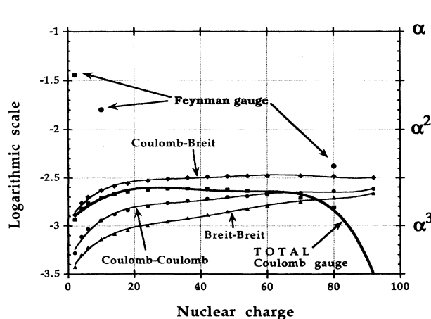
FIG. 7. Same plot as in Fig. 4, but for the part of the QED effects coming from crossed photons. The contribution from the reference state is not included.
