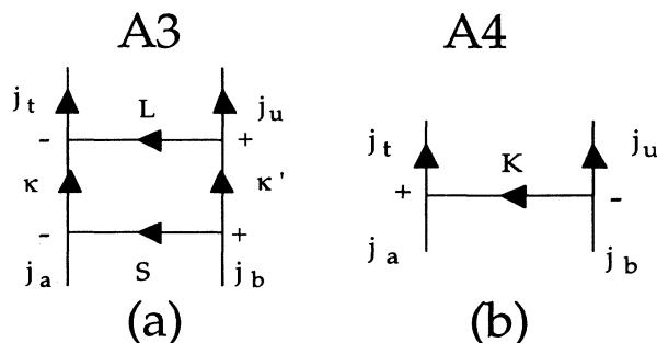
FIG. 10. (a) Angular momentum graph from the reduction of the graph in Fig. 9. (b) Angular momentum graph resulting from further reduction of the graph in (a) when the orbital and spin ranks of the interaction have been coupled to K .
