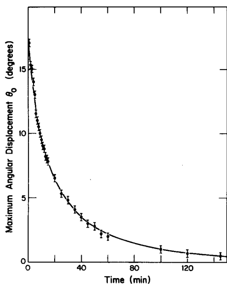
Fig. 2. Decay of amplitude with respect to time. The solid curve is given by Eq. (25) with parameters given by Eqs. (28) and (29). The standard error for a single measurement estimated from the residuals is 0.3^\circ , in agreement with the estimated uncertainty of the observations.
