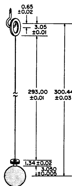
Fig. 1. Dimensions of the pendulum apparatus. Values are given in cm.
