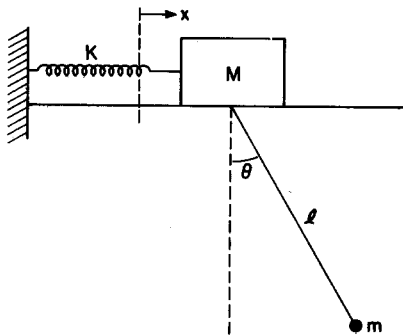
Fig. 3. Model of motion of the support by a system with two degrees of freedom.
