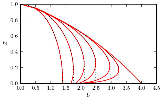
FIG. 2: (Color online) Comparison of results, for two degenerate bands on the 3D cubic lattice with rotational-invariant Hunds interaction, from Gutzwiller (solid lines) and slave-boson 43 (dotted lines), showing the quasi-particle weight \mathcal{Z} as a function of U and (from right to left), J/U = 0, 0.01, 0.02, 0.05, 0.10, 0.20, 0.45 . Additionally, also the higher energy fixpoint solutions of Eq. (88) at finite J/U are reported.
