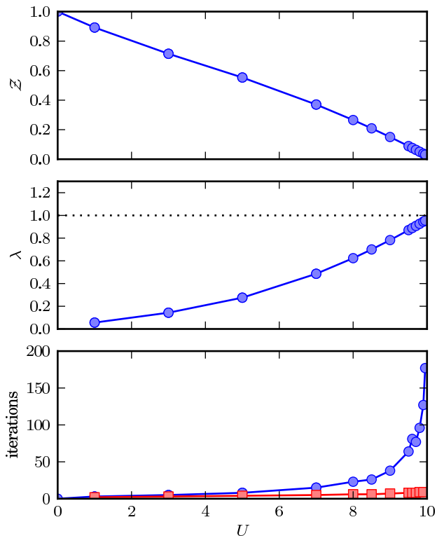
FIG. 6: (Color online) Convergence of the forward recursion scheme (circles) and of the Newton method (squares) for 5 bands at N = 5 , J = 0 and \Delta = 0 . The quasi-particle weight \mathcal{Z} \equiv \mathcal{R}_{\alpha\alpha}^2 goes to zero as U goes to the critical coupling U_c \approx 10 . Simultaneously, the leading eigenvalue \lambda of the Jacobian of the recursion function goes to 1, and the number of forward iterations required to reach a fixed relative precision (here |\mathcal{R}_i - \mathcal{R}_{i+1}| \leq 10^{-6} is used) diverges. On the contrary, the number of Newton iterations is almost independent of U . The matrix [\mathcal{R}_0]_{\alpha\beta} = \delta_{\alpha\beta} is used as initial condition of both the forward recursion series and the Newton method \forall U .
