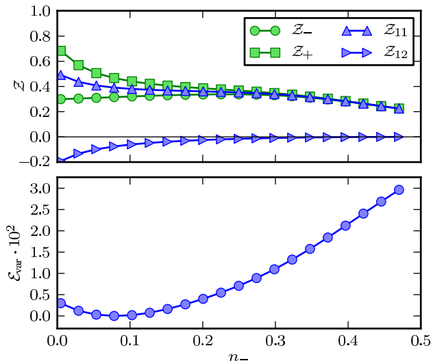
FIG. 7: (Color online) Sweep in the filling of the antibonding orbital n_- for the two-bands bilayer Hubbard model with equal bandwidths, local hybridization V = 0.25 , filling N = 1.88 , U' = J' = J = 0 and U = 2.5 . Renormalization matrix Z (top panel) and total energy (bottom panel).
