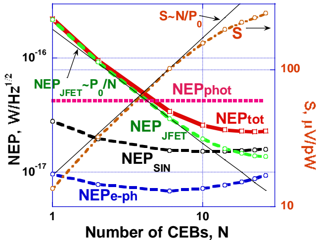
Figure 4. NEP components and photon NEP in dependence on the number of CEBs in a series array. The parameters of CEBs are the same as in figure 3. The responsivity S is shown for illustration of the effect of CEB number. Thin lines show asymptotics for S (10) and NEP_{JFET} (11).
