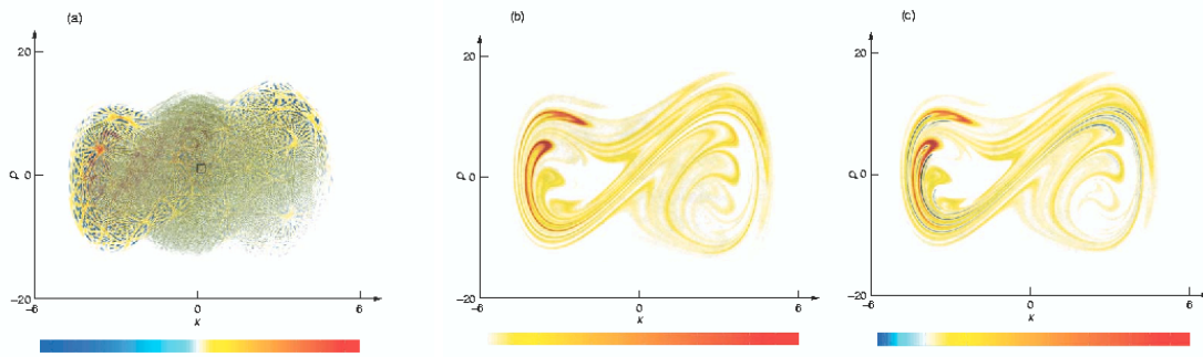
Figure B: Decoherence in a Chaotic Driven Double-Well System. This numerical study (Habib et al. 1998) of a chaotic driven double-well system described by the Hamiltonian H = p^2/2m - Ax + Bx^4 + Fx \cos(\omega t) with m = 1, A = 10, B = 0.5, F = 10 , and \omega = 6.07 illustrates the effectiveness of decoherence in the transition from quantum to classical. These parameters result in a chaotic classical system with a Lyapunov exponent \lambda \cong 0.5 . The three snapshots taken after 8 periods of the driving force illustrate phase space distributions in (a) the quantum case, (b) the classical case, and (c) the quantum case but with decoherence ( D = 0.025 ). The initial condition was always the same Gaussian, and in the quantum cases, the state was pure. Interference fringes are clearly visible in (a), which bears only a vague resemblance to the classical distribution in (b). By contrast, (c) shows that even modest decoherence helps restore the quantum-classical correspondence. In this example the coherence length \ell_C is not much smaller than the typical nonlinearity scale, so the system is on the border between quantum and classical. Indeed, traces of quantum interference are still visible in (c) as blue “troughs,” or regions where the Wigner function is still slightly negative. The change in color from red to blue shown in the legends for (a) and (c) corresponds to a change from positive peaks to negative troughs. In the ab initio classical case (b), there are no negative troughs.
