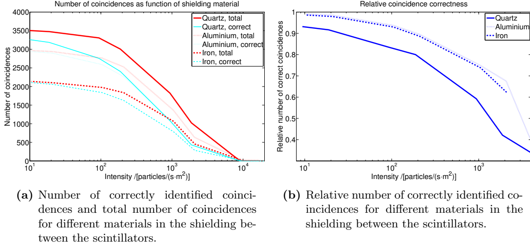
Figure 18: Correct and incorrect coincidences for different shielding materials.
