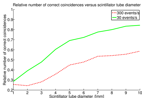
Figure 17: Relative number of correct coincidences as function of tube diameter. The number of events per second is approximate, and varies from about 15 % lower for the smallest scintillator tube size due to a decreased number of detected decays when the scintillator diameter becomes smaller. The average frequency of fired, detected particles is however the same for each curve. An alternative to holding the number of events per second fixed would be to fix the number of events per second per area unit.
