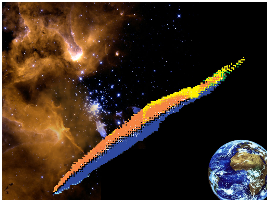
Fig. 1. Atomic nuclei be organised in a grid of squares, each of which represents a certain number of protons (vertically) and neutrons (horizontally), together forming the chart of nuclides, as shown here. This chart, or nuclear landscape, is the working field of ISOLDE, where the main emphasis is the most exotic nuclei. The nuclei studied at ISOLDE give important new insight in the complex nuclear many-body system. They give clues to the simplicity hidden in the complexity, they tell us about the elements that build up the nature around us and about their cosmic origin and plays a prominent role in our understanding of the formation of the chemical elements.
