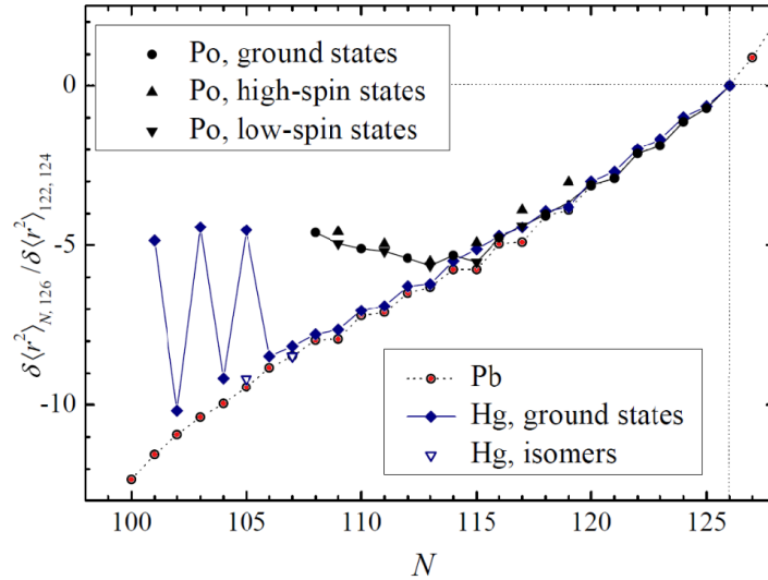
Fig. 8. Relative change in mean-square nuclear charge radii, \delta \langle r^2 \rangle , for the even- Z ^{80}\text{Hg} (blue), ^{82}\text{Pb} (red) and ^{84}\text{Po} (black) isotopes. While the relative change in charge radii of one isotope compared to its neighbour for the heaviest isotopes are very similar for these three elements, large differences are observed further away from the N=126 neutron shell closure. The large staggering observed in the Hg data is interpreted as shape coexistence caused by the occupation of specific single-particle states. The deviation observed for the Po isotopes is linked to an onset of collective behaviour possibly caused by the same mechanism. Adapted from Ref. 18
