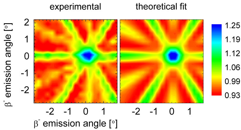
Fig. 5. Emission channeling data recorded using a position sensitive silicon detector. The colour scale corresponds to the angular dependent yield of channeled beta particles emitted from radioactive ^{56}\text{Mn} probes implanted into a GaAs (semiconductor) sample. 11 The data (left) are fitted to simulations (right) from which the site location of Mn in the GaAs matrix can be determined enhancing the understanding of electrical, optical and magnetic influence of dopants in semiconductors.
