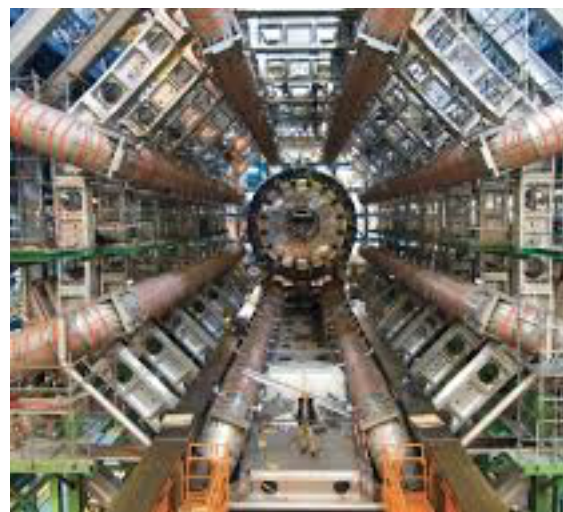
Higgs
