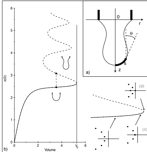
FIG. 1. a) Definition of the variables characterizing the drop. b) The dimensionless length z(0) versus the dimensionless volume V of the drop. The dashed line corresponds to unstable stationary drops, the solid line to the stable drops. V_c \approx 5.20 is the maximum volume of a stationary pendant drop. On the right we show the corresponding eigenvalue spectrum for some representative points close to V_c ; the onset of the saddle-node bifurcation is shown in (2), and the leading eigenvalues are \lambda_1 = 0, \lambda_2 = -0.017 \pm i.3.468 .
