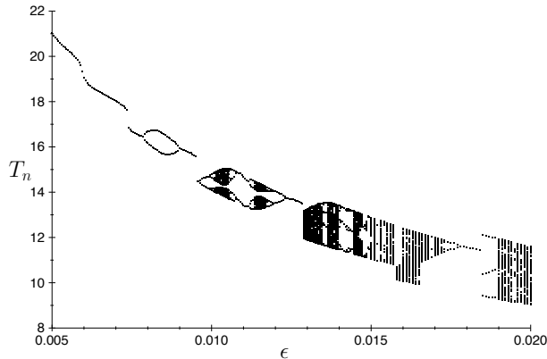
FIG. 4. A phase diagram corresponding to the changes in the dripping behavior as a function of the flow rate \epsilon , computed using the return map (12). Very similar diagrams are obtained by solving (5) numerically [7]. For small and large flow rates, the dripping is periodic. For intermediate flow rate, the dripping may be chaotic. The transition to chaos occurs by either a period doubling bifurcation, e.g. \epsilon = 0.01 , or the result of boundary crisis, e.g. \epsilon = 0.0125 . For this simulation, the scaled damping rate \lambda = .17 , and the scaled frequency \omega = 3.46 .
