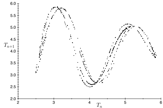
FIG. 5. A return map corresponding to the discrete dynamical system (12), showing the time interval between two consecutive drops T_{n+1} versus the previous such interval T_n , for the same parameters as in FIG. 5. This attractor is characteristic of chaos in the dripping faucet experiment [18,19].
