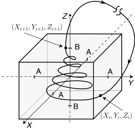
FIG. 3. A parallelepiped around the saddle point in phase-space is used to construct the mapping from the plane before the bifurcation to the plane after the bifurcation. A simple rigid rotation is used to model the global reinjection process associated with the complex dynamics of pinch-off, recoil and growth.
