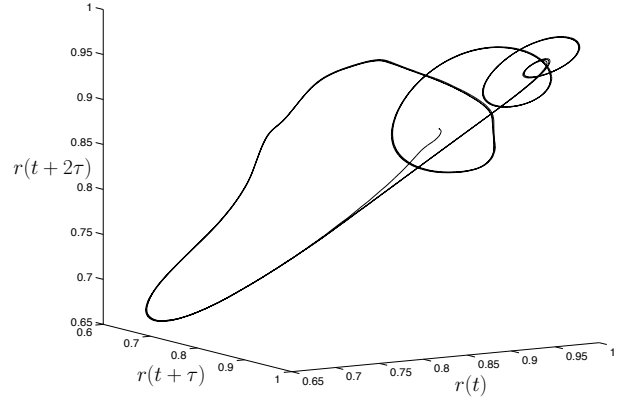
FIG. 2. Reconstruction of the flow by the time delay method, obtained by solving (5) numerically. The radius of the drop is probed at the location z = 0.5 and is always continuous. The parameters used for the simulation correspond to a fluid 10 times more viscous than water flowing out of a faucet of diameter R = 1 at a flow rate \epsilon = 0.01 (in dimensional terms, R = 2.6mm, \epsilon = 0.015cm^3/s ). We observe a long excursion followed by a damped oscillations before the orbit returns to the neighborhood of the saddle point.
