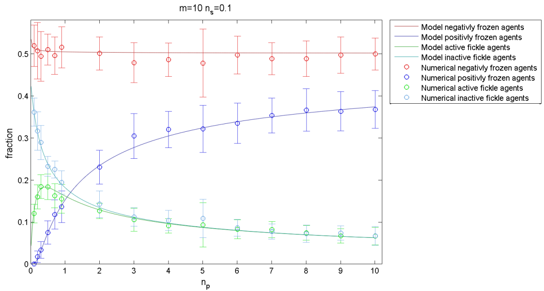
Figure 7: With parameters m = 10 and n_s = 0.1 , we can see how well the characteristics of the model and numerical simulations correspond. Numerical data is the average over twenty simulations and the standard deviation is plotted to visualize the rather small deviations.
