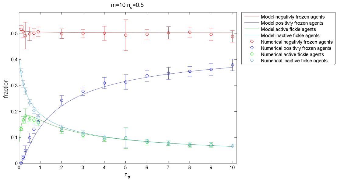
Figure 9: With parameters m = 10 and n_s = 0.5 , we can see how well the characteristics of the model and numerical simulations correspond. Numerical data is the average over twenty simulations together with standard deviation. With larger m the simulations get smaller standard deviations.
