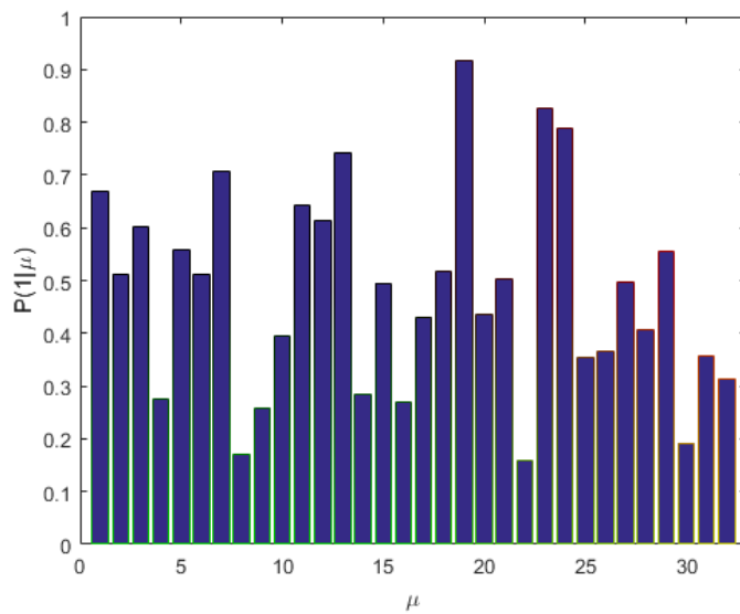
Figure 3: Histogram of conditional probability of choosing the bid 1 given a specific history for \alpha = \frac{2^5}{51} > \alpha_c .
