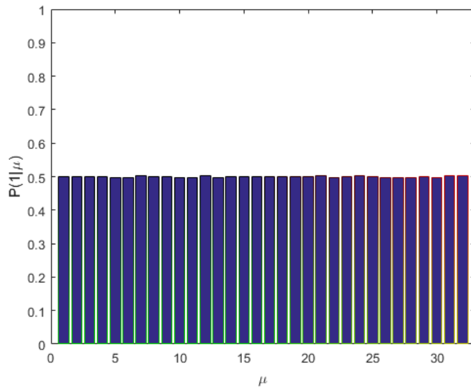
Figure 2: Histogram of conditional probability of choosing the bid 1 given a specific history for \alpha = \frac{2^5}{501} < \alpha_c .
