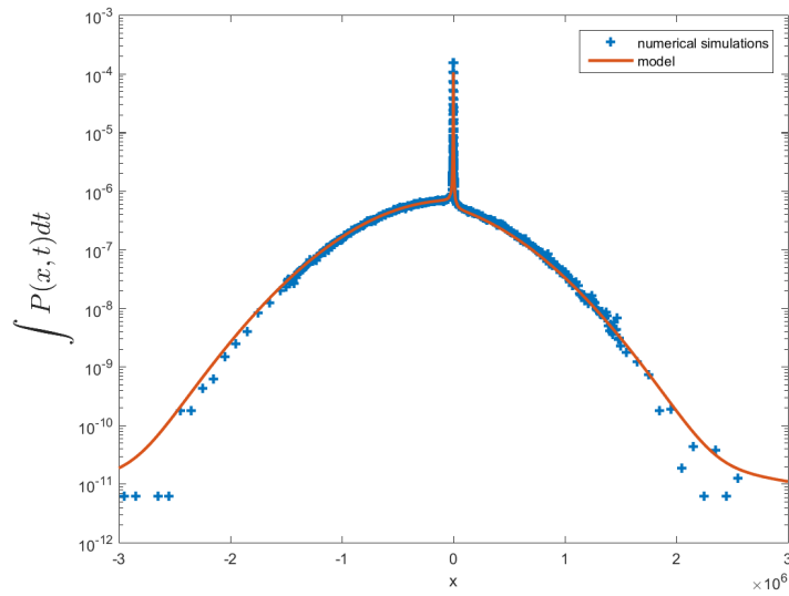
Figure 14: Full score distribution integrated over a time window t_0 = 4 \cdot 10^5 to t_1 = 5 \cdot 10^5 with parameters m = 8, n_s = 0.5 and n_p = 2 . The agreement to model values is very good. To note, there is only a few values for the tails, and the model under predicts close to x = 0 . The numerical data is from 12600 runs with the above parameters.
