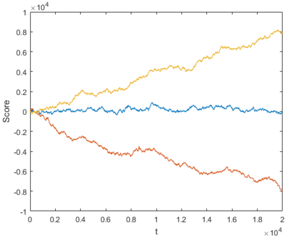
Figure 6: Here we have taken out the three agents with different characteristics from the above simulation. We see that after a time, the yellow agent is always active (score over zero), the blue one are occasionally active (score around zero) and the red one is never active (score under zero).
