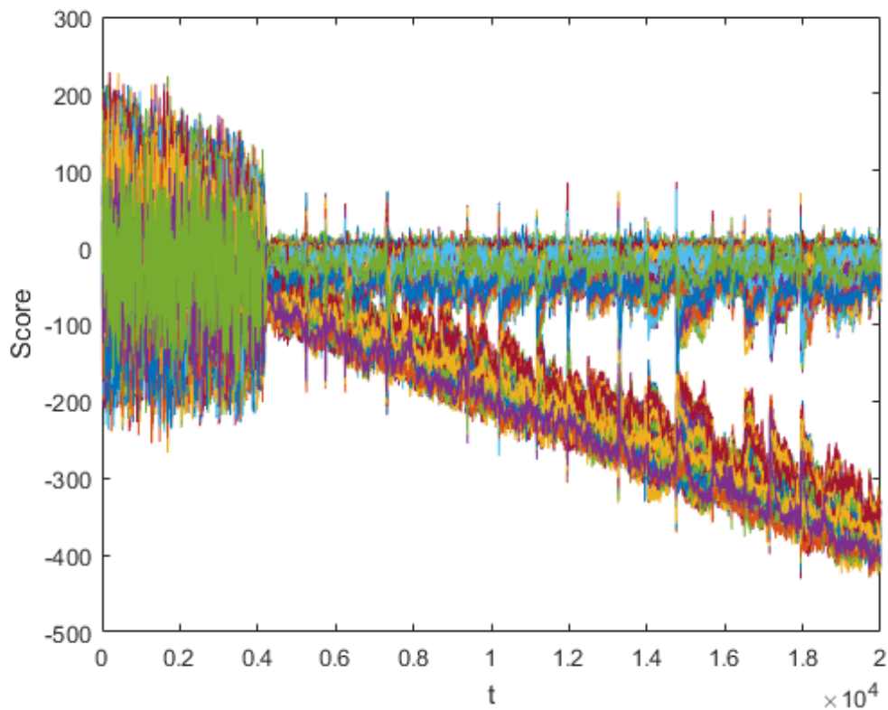
Figure 4: Here we can see a realization of the game for m = 4 and N = 20P . We can clearly see the strategies dividing in two distinct groups. We also note spikes in strategy scores which happens fairly regularly.
