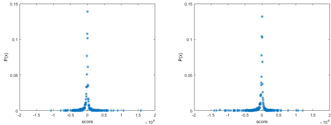
(a) Numerical score distribution for fickle agents at time t = 3.5 \cdot 10^6 . (b) Numerical score distribution for fickle agents at time t = 4 \cdot 10^6 .
