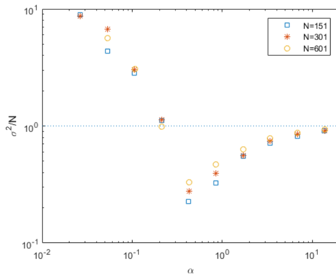
Figure 1: Here we can see the phase transition. For small \alpha we have a large volatility whereas for larger values we get close to the coin-toss limit. Every point is averaged over 5 runs of 10^4 time steps.
