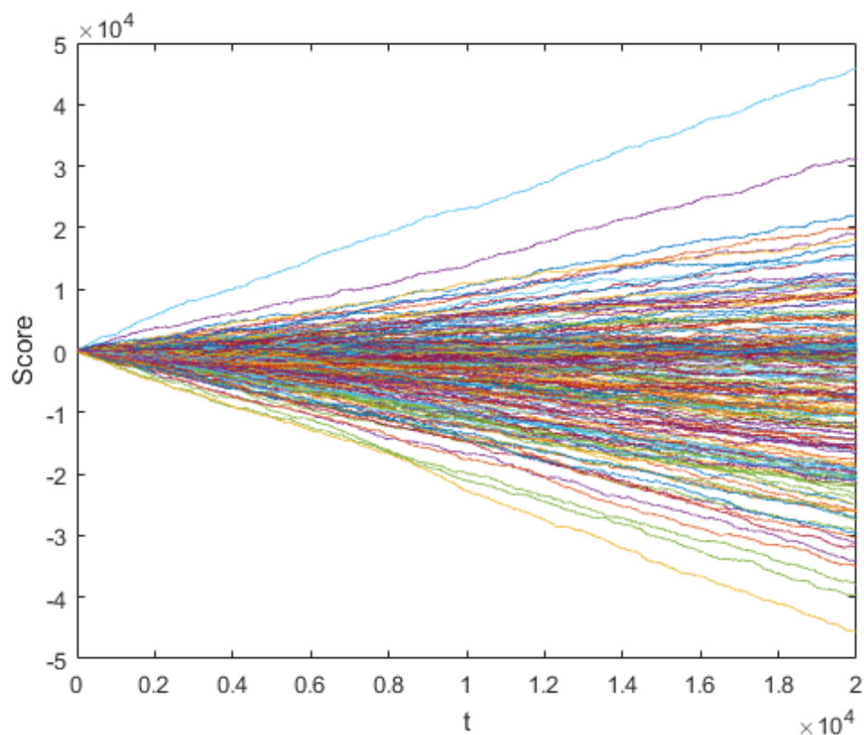
Figure 5: Here we can see a realization of the game for m = 8 and N_s = P . We see that we do not have the same effects as above. We note that the strategies generally seem to loose points.
