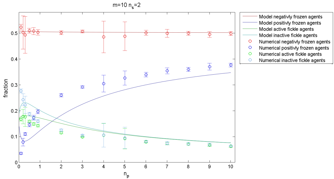
Figure 11: With parameters m = 10 and n_s = 2 , we can see how well the characteristics of the model and numerical simulations correspond. Numerical data is the average twenty simulations together with standard deviation. We note that for n_s = 2 the model is quite a bit off, and you can clearly see how it is qualitatively different for small n_p .
