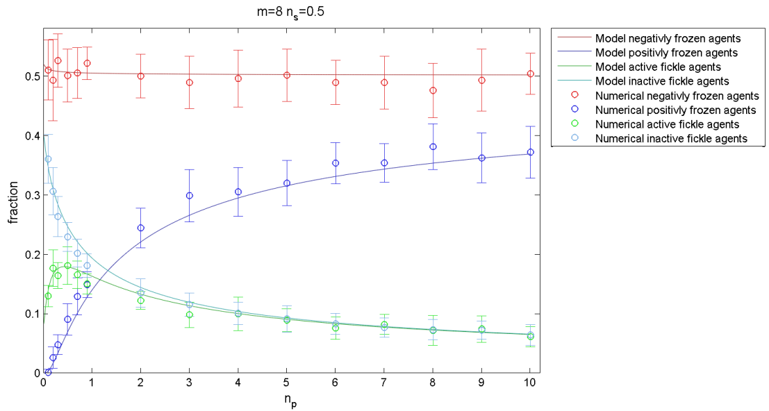
Figure 8: With parameters m = 8 and n_s = 0.5 , we can see how well the characteristics of the model and numerical simulations correspond. Numerical data is the average over twenty simulations and the standard deviation is plotted to visualize the rather small deviations.
