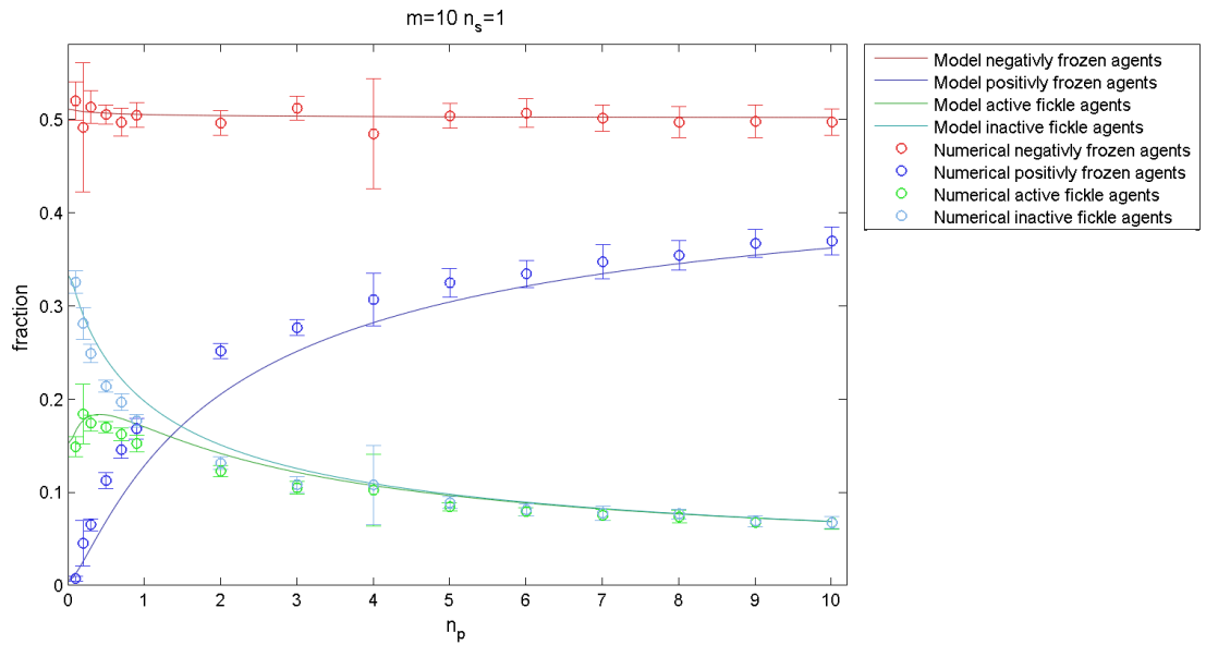
Figure 10: With parameters m = 10 and n_s = 1 , we can see how well the characteristics of the model and numerical simulations correspond. Numerical data is the average over twenty simulations together with standard deviation.
