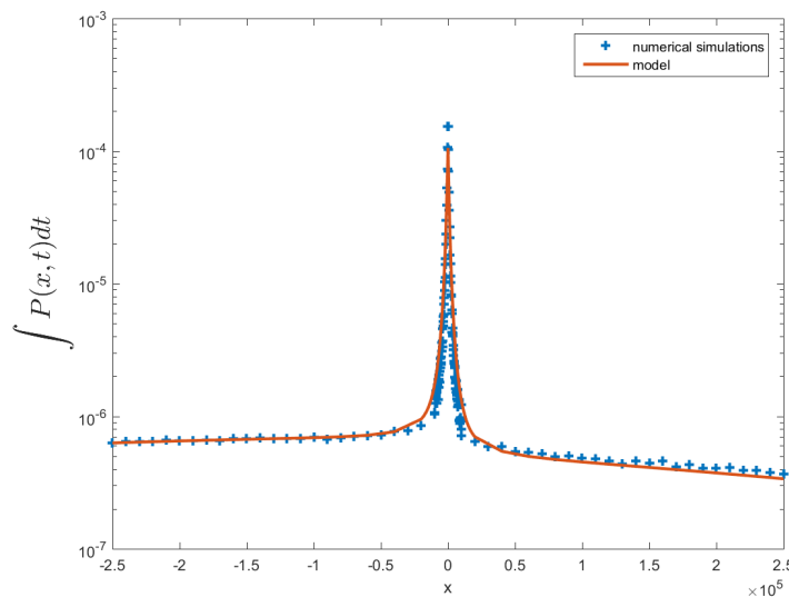
Figure 15: Here we see a full score distribution zoomed in around x = 0 . Here we clearly see that it under predicts the probability of very small values of x .
