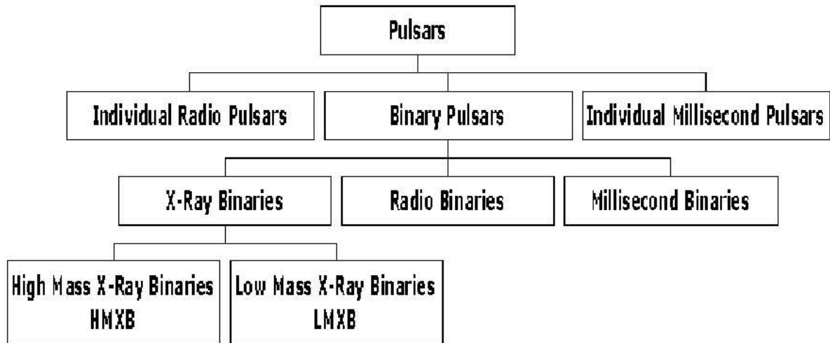
Figure 3: The classification of pulsars
